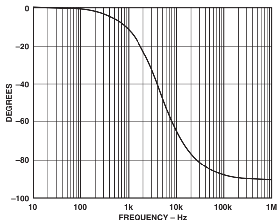
Figure 8. RC Filter Phase Response
