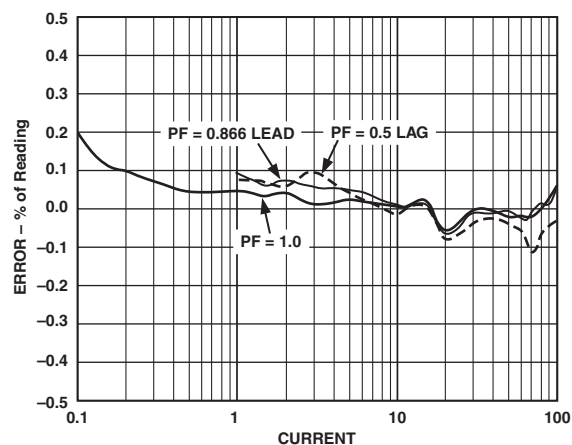
Figure 15. AC Linearity Error
