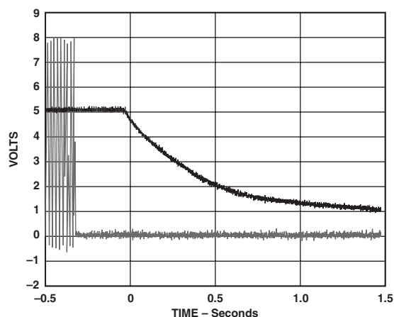
Figure 13. Power Supply Droop
