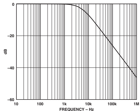
Figure 7. RC Filter Magnitude Response
