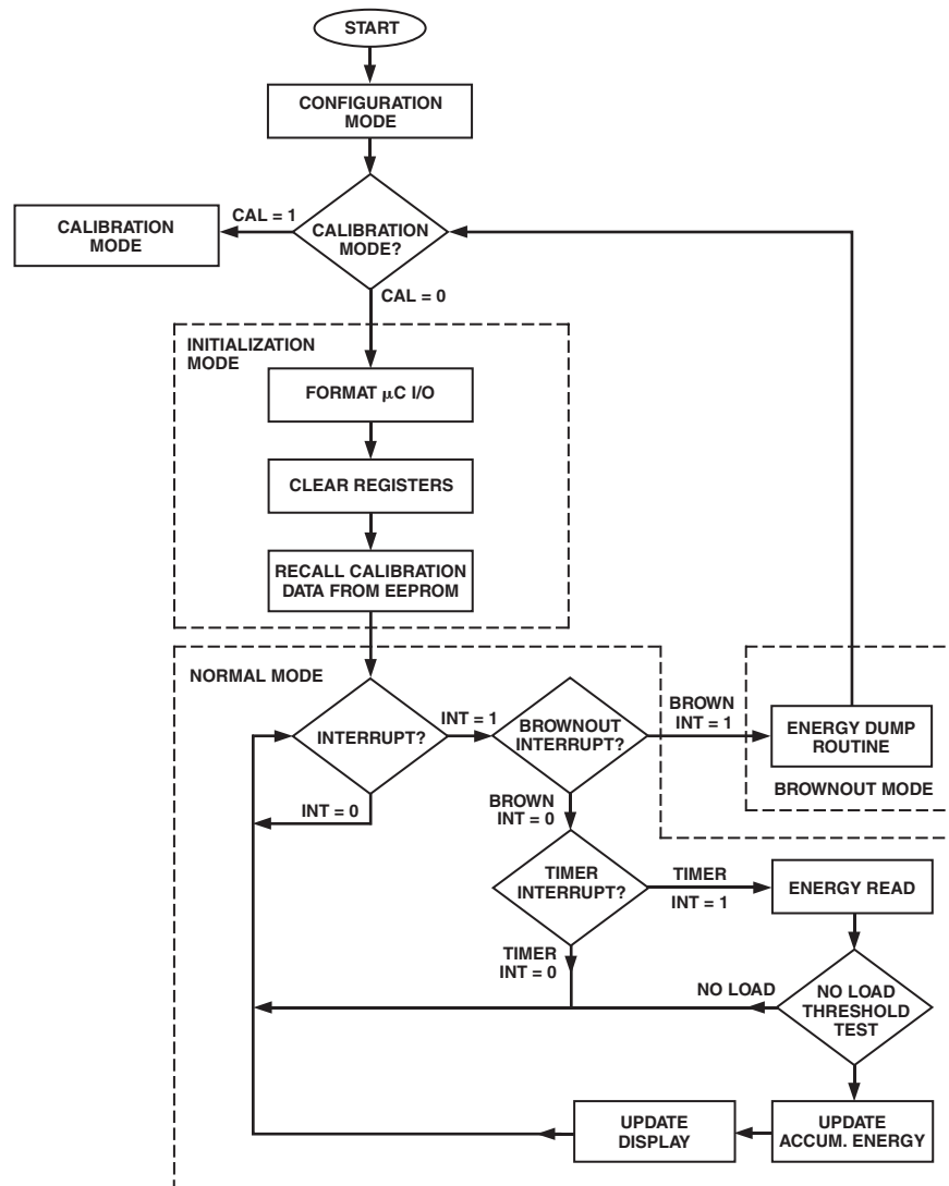
Figure 14. Program Flow Chart
