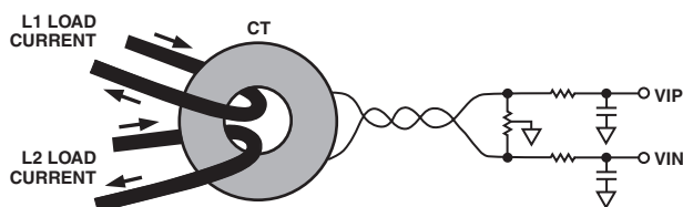
Figure 3. ADE7756 CT Wiring Diagrams
