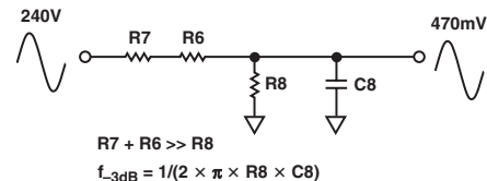
Figure 4. Attenuation Network
