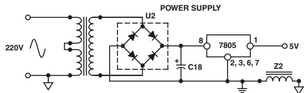
Figure 10. Power Supply
