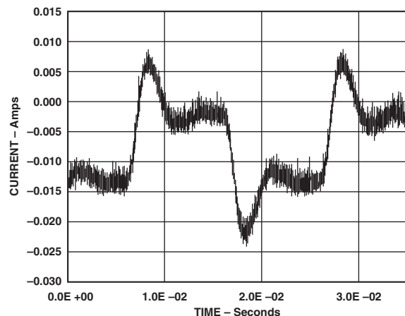
Figure 11. Power Supply Current
