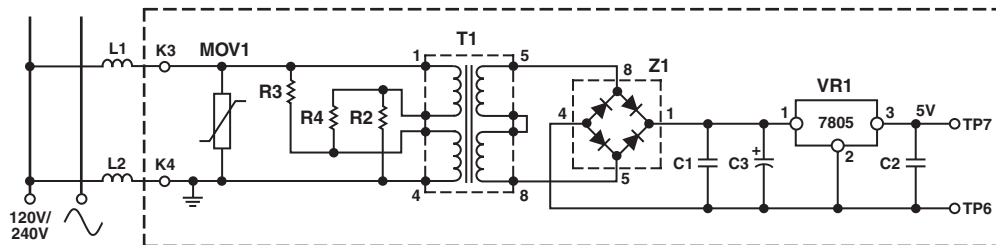
Figure 17. Reference Design Power Supply
