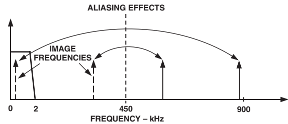
Figure 6. Aliasing Effects
