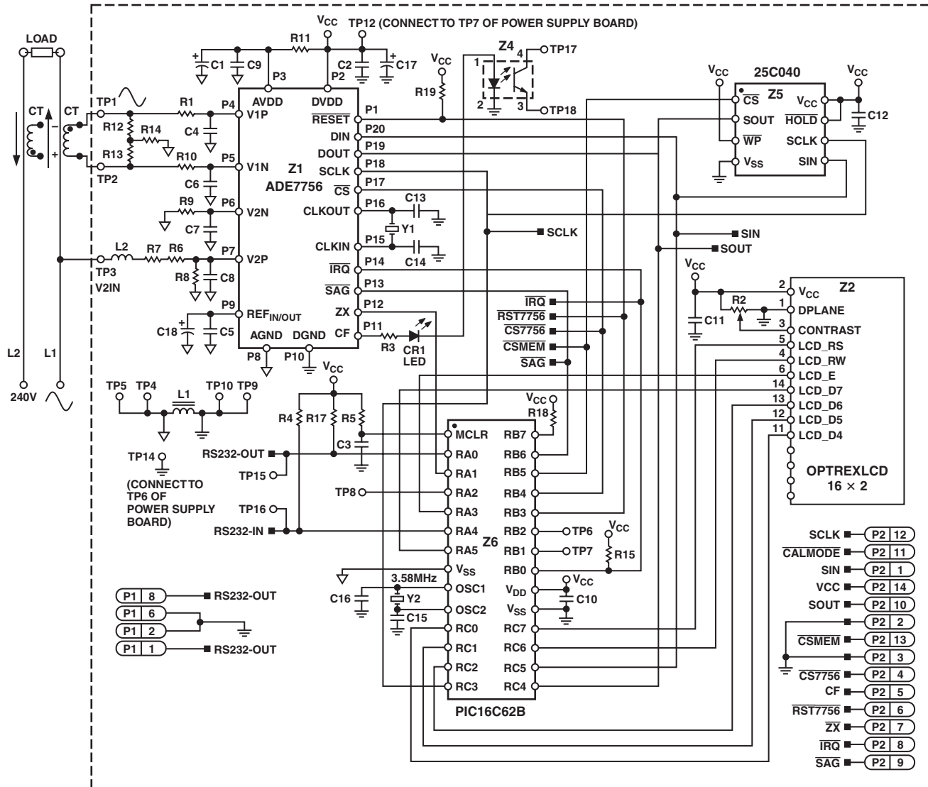
Figure 16. Reference Design Schematic
