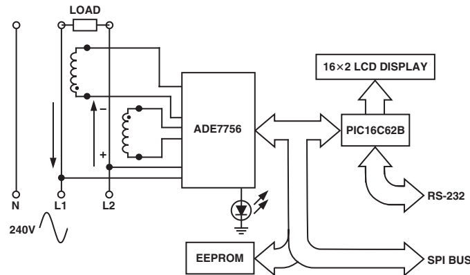
Figure 1. Simple Single Phase Watt-Hour Meter Block Diagram
