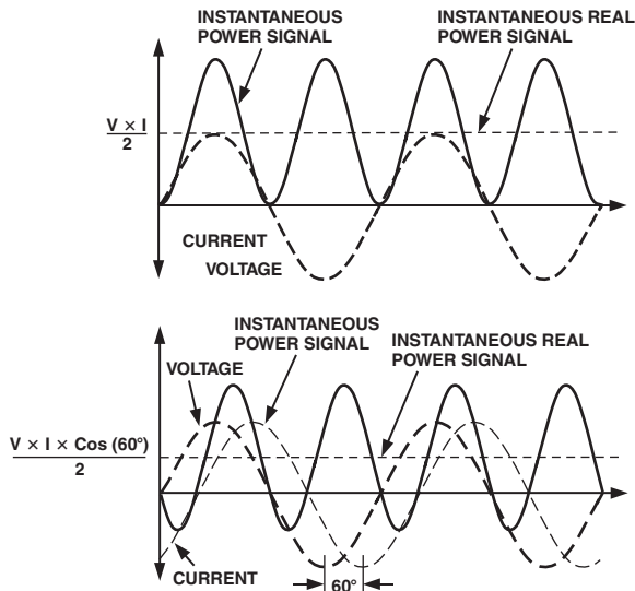
Figure 5. Voltage and Current (Inductive Load)
