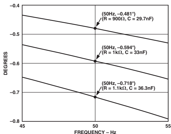
Figure 9. Phase Shift at 50 Hz Due to Component Tolerances
